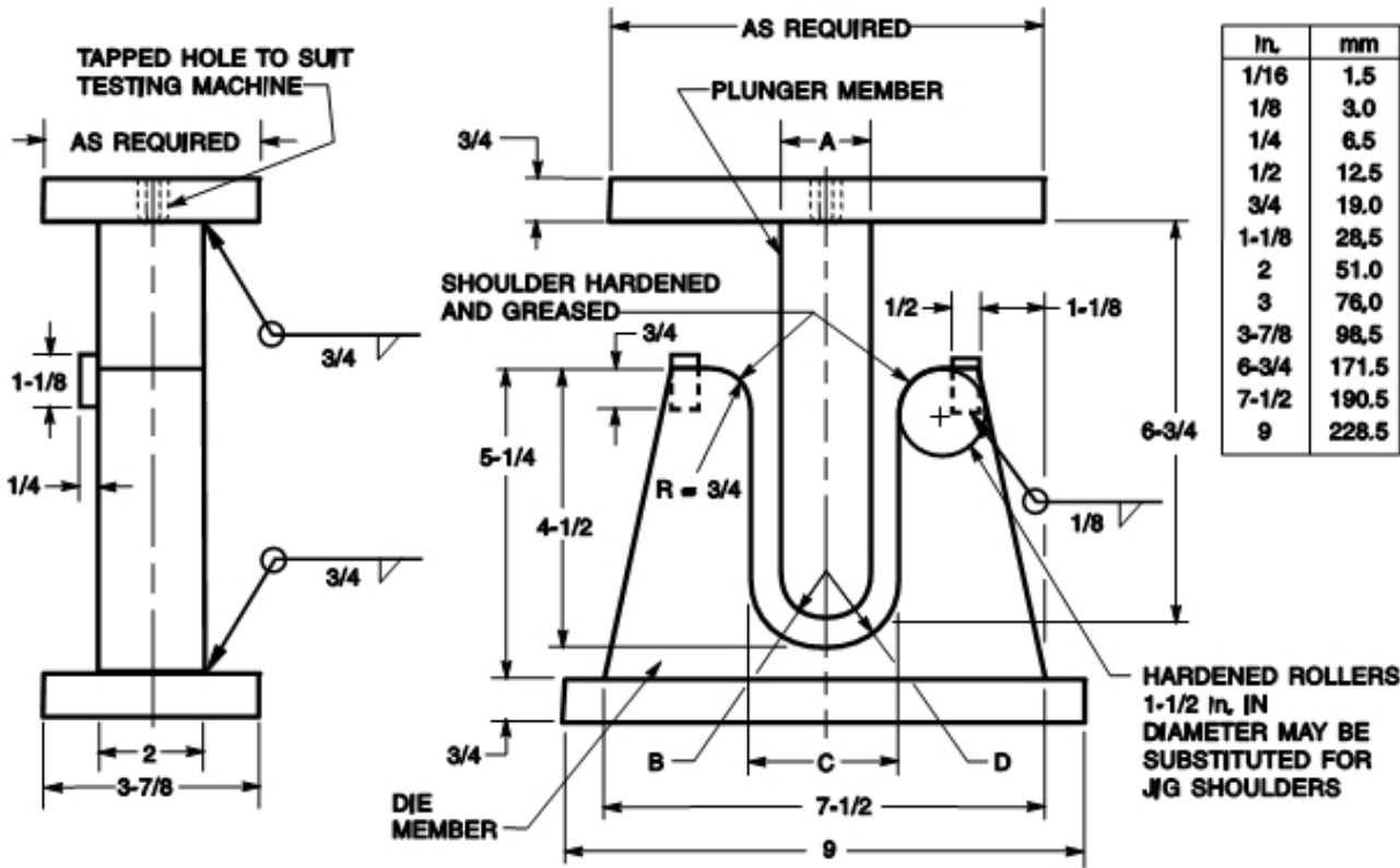
Figure 2—Guided-Bend Test Jig
